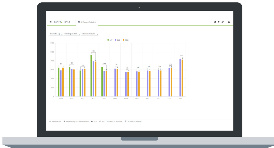
Fig. 2 Forecast Analysis
